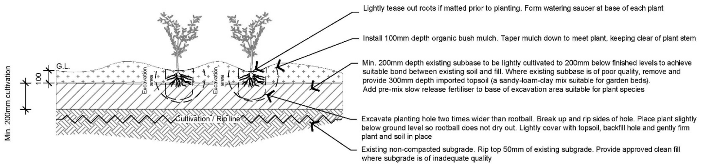
01 GARDEN BED INSTALLATION Section 1:20
