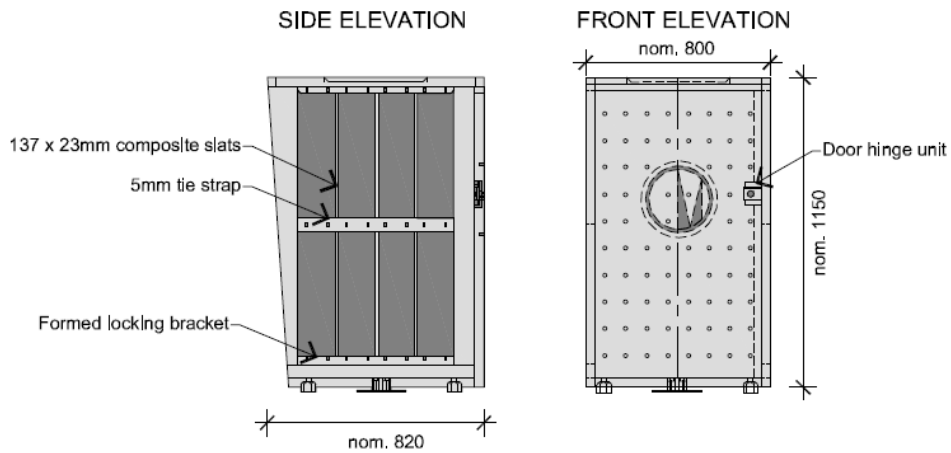
03 PARKS BIN SURROUND Elevation views 1:20
