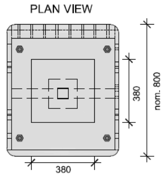
02 PARKS BIN SURROUND Plan view 1:20
