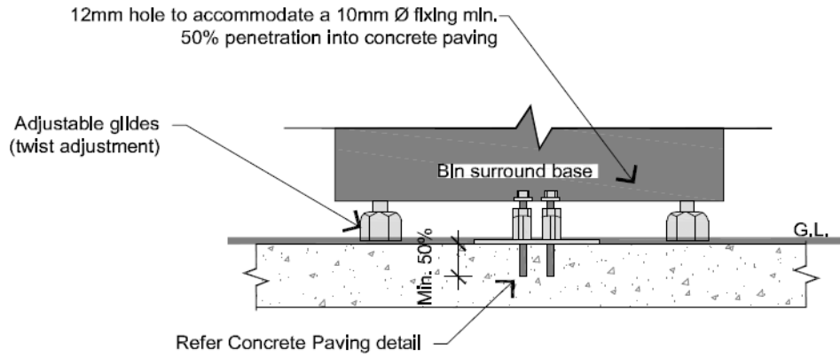
01 PARKS BIN SURROUND FIXING Side Elevation 1:10
