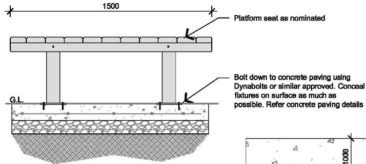
01 PARKS PLATFORM SEAT Side Elevation 1:20
