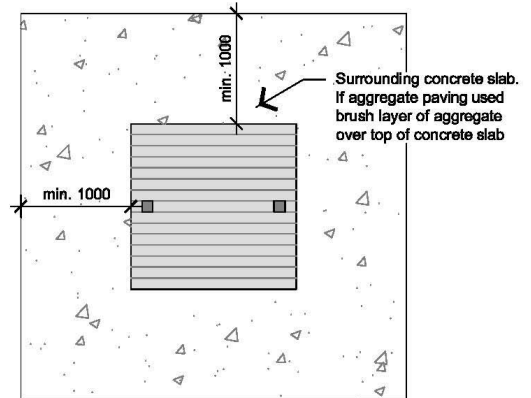
02 PARKS PLATFORM SEAT Plan View 1:50
