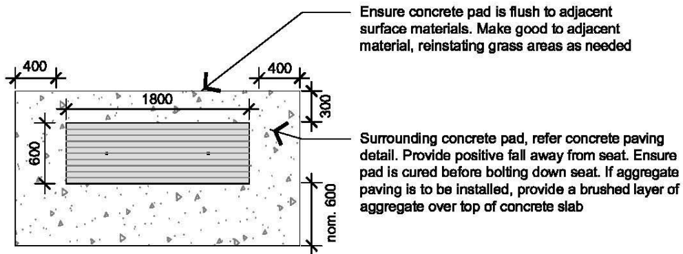
02 PARK BENCH Plan View 1:50
