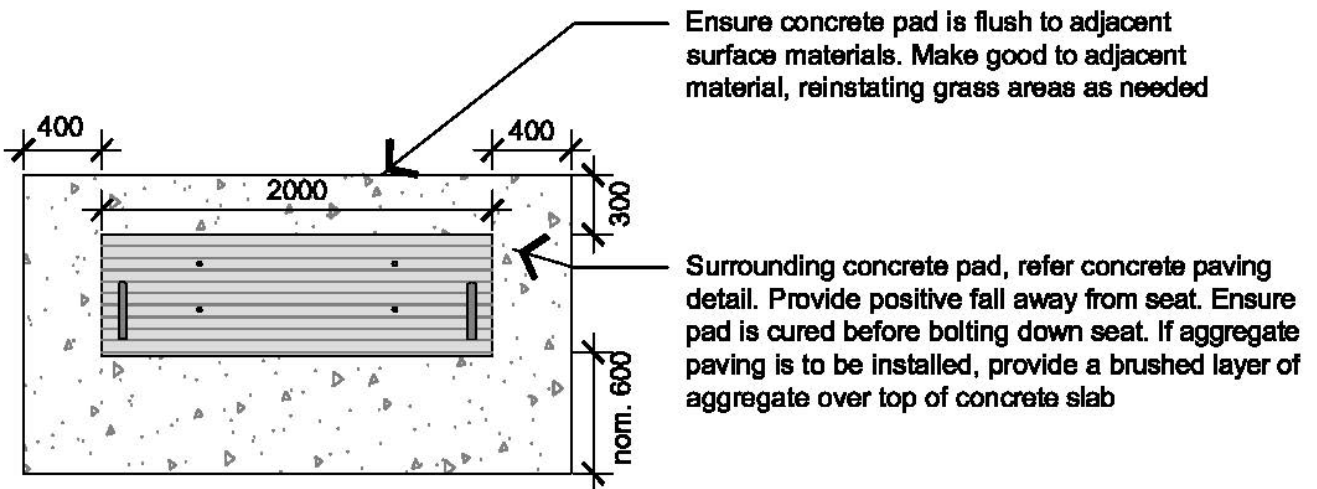
02 PARKS SEAT Plan View 1:50
