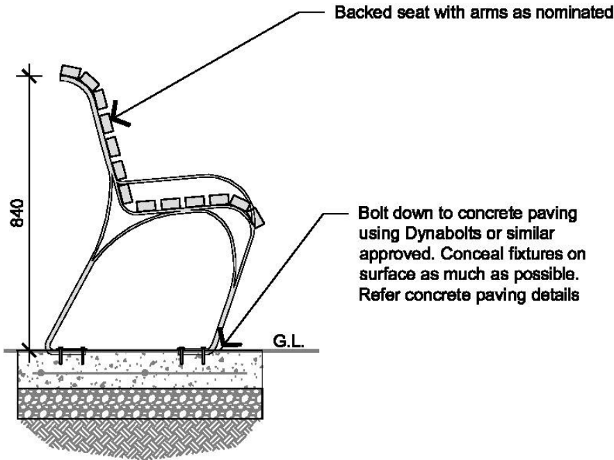
01 PARKS SEAT Side Elevation 1:20
