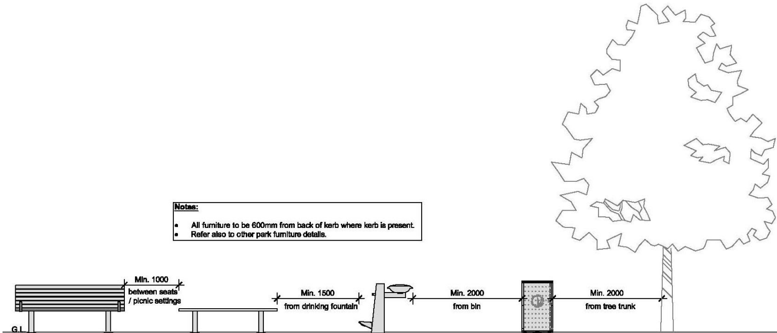
01 PARK FURNITURE LAYOUT Front Elevation 1:50
